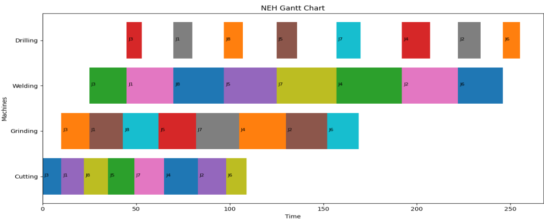
Fig. 3 NEH Gantt chart
