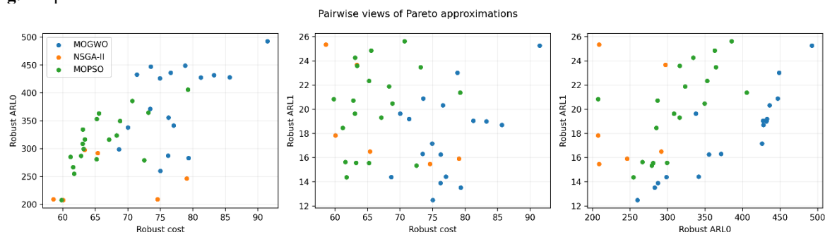
Fig. 2 Optimized Pareto solutions in three different dimensions
