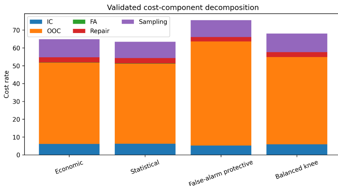
Fig. 6 Decomposition of the validated and optimized cost into In-Control (IC), False Alarm (FA), Sampling, Out-of-Control (OOC) and Repair cost.
