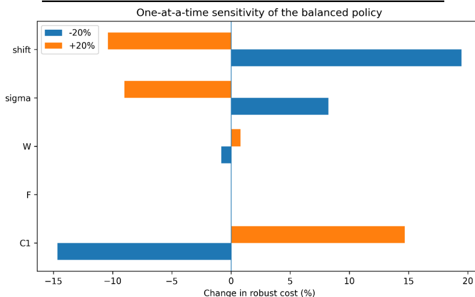
Fig. 7 Results of the impact of main parameters changes on the robust costs and statistical measures
