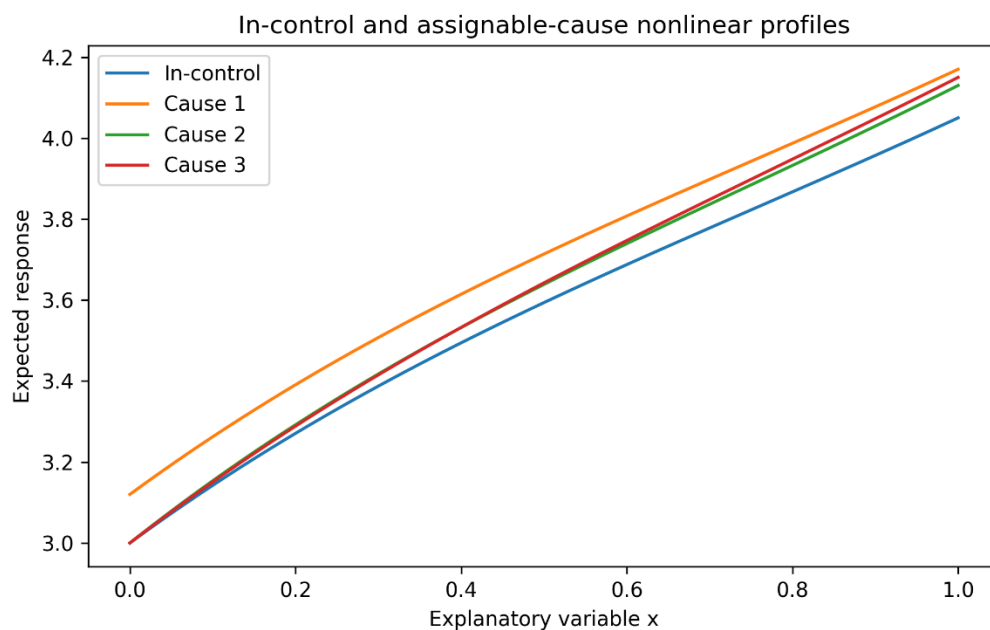
Fig. 1 In-control profile and three different cause-specific nonlinear profile
