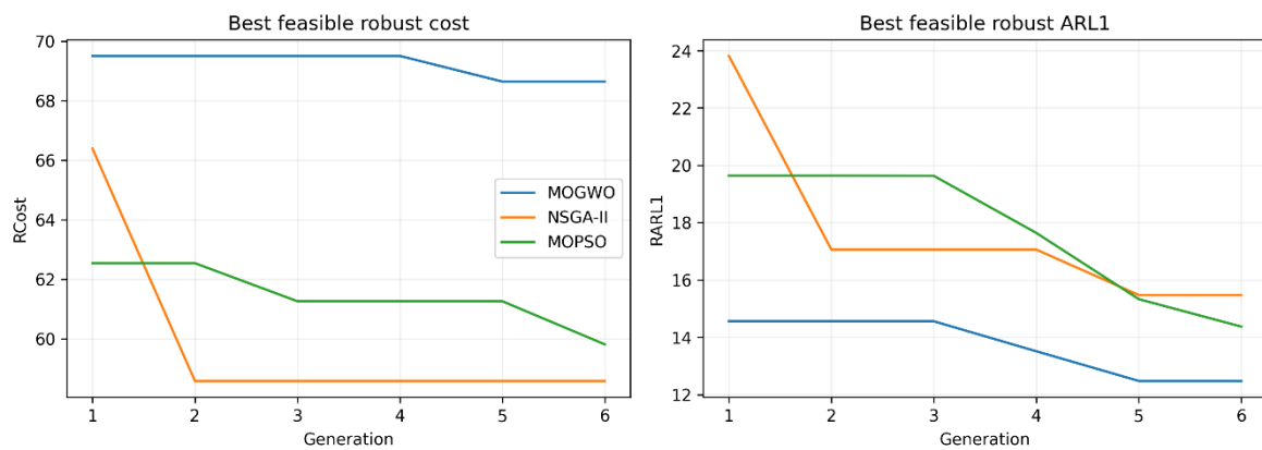
Fig. 5 Comparative evaluation of three methods based on evolution rate of feasible robust cost and feasible robust ARL1
