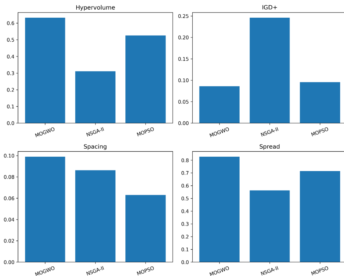
Fig. 4 Comparative results on three meta-heuristics methods based on HV, IGD+, Spacing and Spread measures
