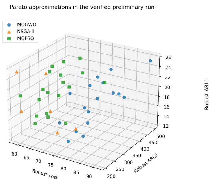
Fig. 2 Optimized Pareto solutions in three different dimensions
