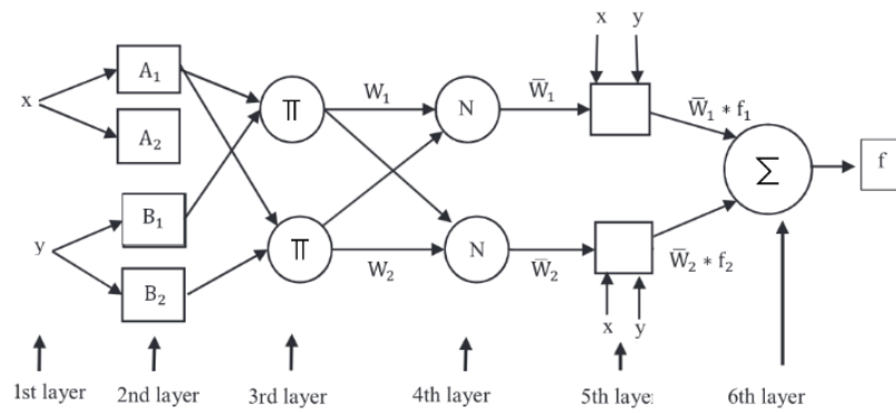
Fig. 1 ANFIS structure with two inputs
