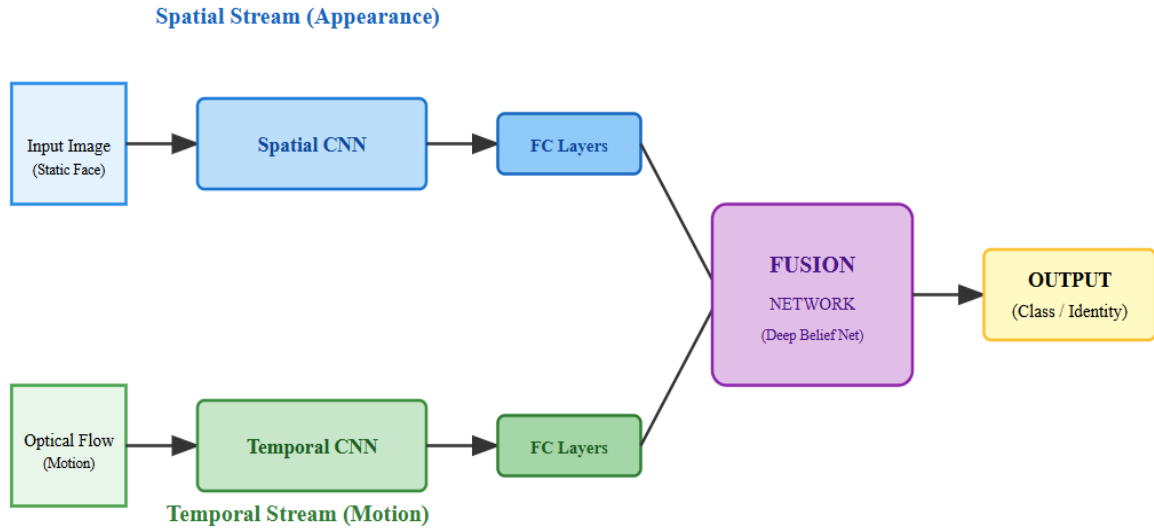
Fig. 3 Architecture of the Dual-Stream Convolutional Neural Network (CNN) for Facial Analysis.
