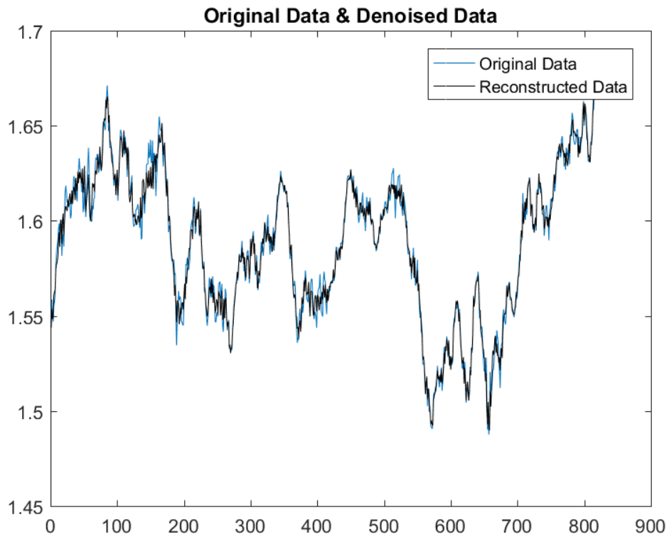
Fig. 15 Denoising GBP/USD with EMD
