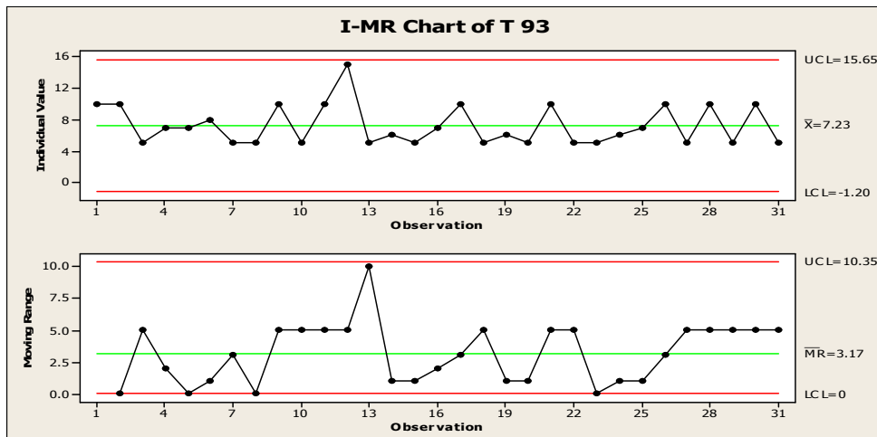
Fig. 8 I-MR chart
