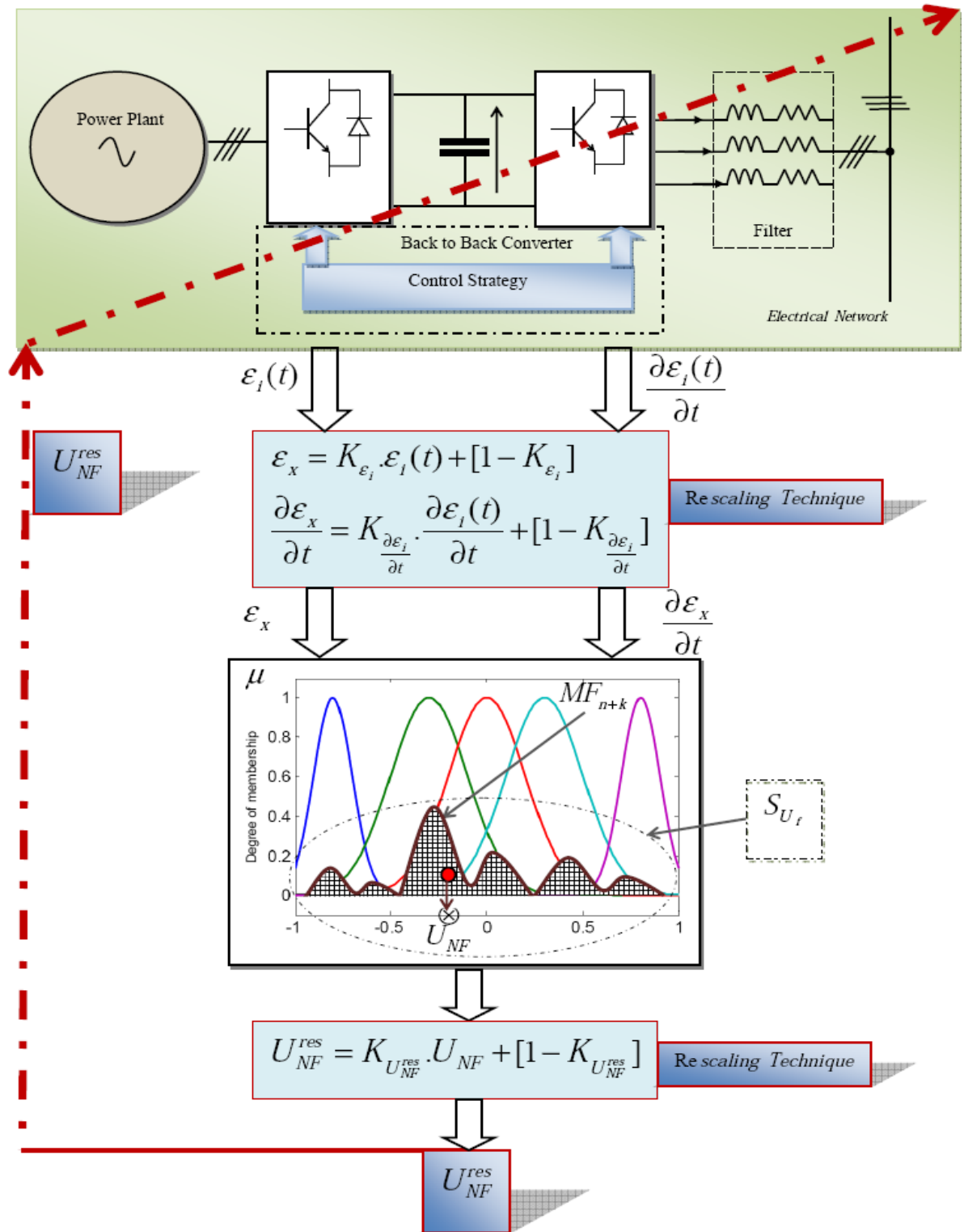
Fig. 5 Rescaling flowchart
