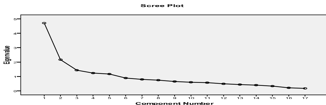
Fig. 1 Scree Plot
